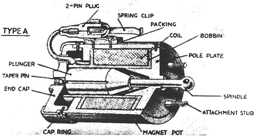
FIRING SOLENOIDS FOR BROWNING GUNS
